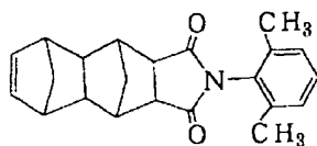
Structural formula (E) :
