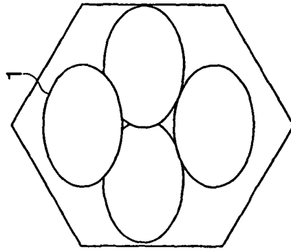
CAPSID STRUCTURE
