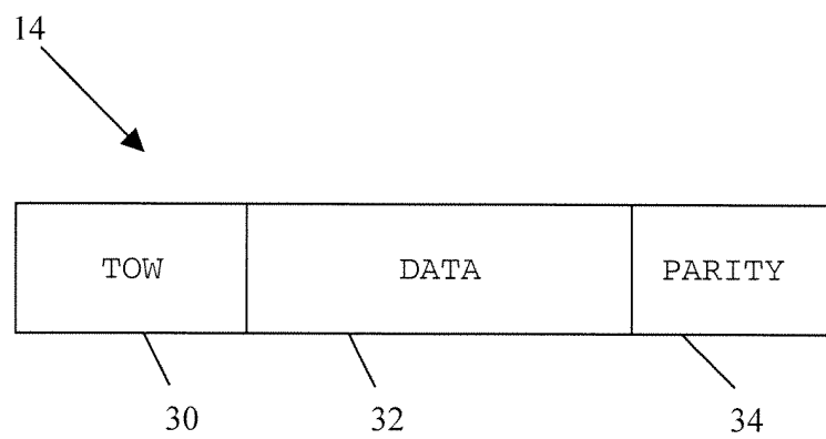
Figure 3 (Prior Art)
