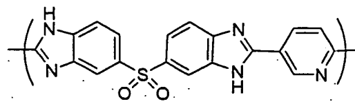
Chemical Formula 8-2
