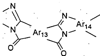
(Chemical Formula 26)
