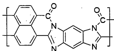
Chemical Formula 27-1
