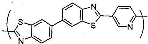
Chemical Formula 8-5
