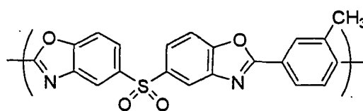
Chemical Formula 9-4
