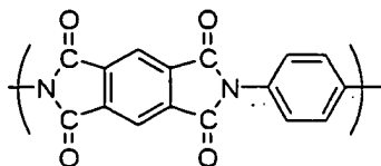
Chemical Formula 15-1
