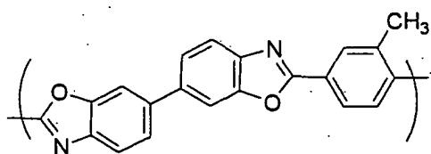
Chemical Formula 9-3
