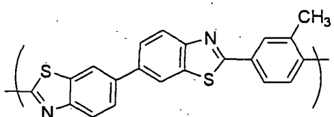
Chemical Formula 9-5
