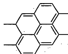
Chemical Formula 13-8
