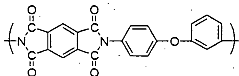
Chemical Formula 15-3
