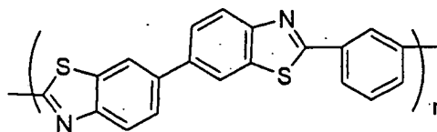
Chemical Formula 7-6
