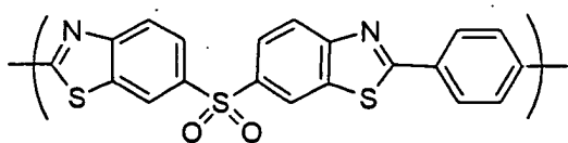
Chemical Formula 7-11
