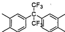
Chemical Formula 13-6
