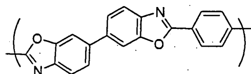
Chemical Formula 7-3
