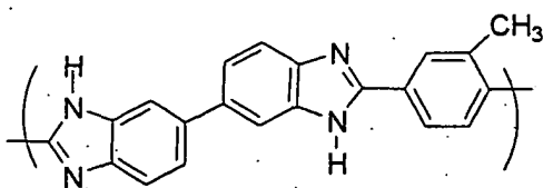
Chemical Formula 9-1
