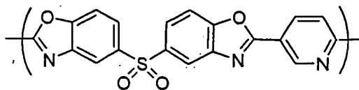
Chemical Formula 8-4
