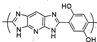
Chemical Formula 10-6
