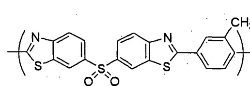
Chemical Formula 9-8
