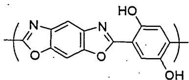
Chemical Formula 10-1
