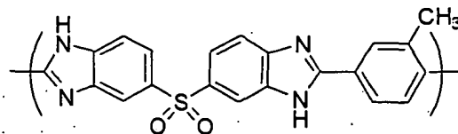
Chemical Formula 9-2
