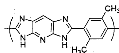
Chemical Formula 6-8
