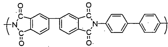
Chemical Formula 15-8
