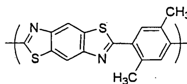
Chemical Formula 6-6
