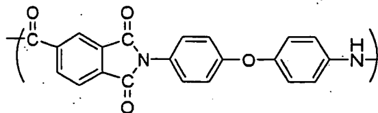
Chemical Formula 21-2
