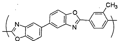
Chemical Formula 9-7
