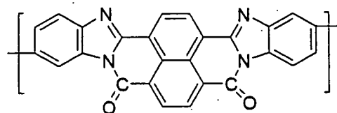
Chemical Formula 27-2
