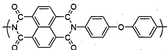
Chemical Formula 16-5
