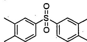
Chemical Formula 13-4
