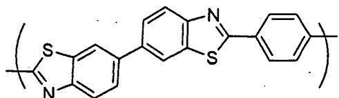
Chemical Formula 7-5
