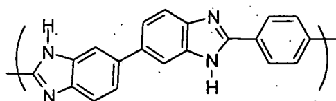
Chemical Formula 7-1
