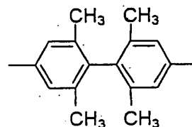
Chemical Formula 3-12
