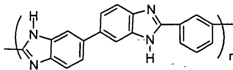
Chemical Formula 7-2
