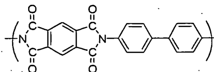
Chemical Formula 15-2
