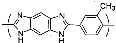
Chemical Formula 6-3
