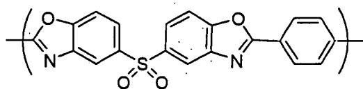
Chemical Formula 7-9
