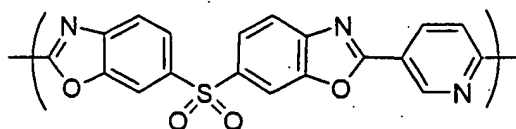
Chemical Formula 8-6
