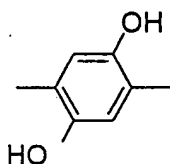
Chemical Formula 3-7
