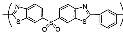
Chemical Formula 7-12
