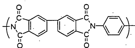
Chemical Formula 15-5
