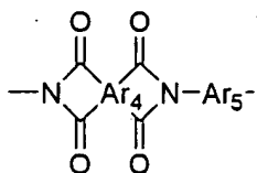
(Chemical Formula 12)
