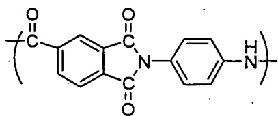
Chemical Formula 21-1
