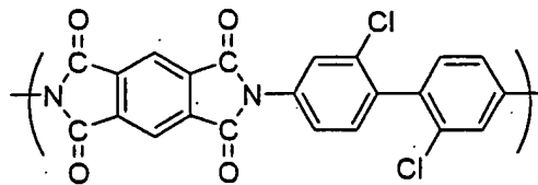
Chemical Formula 16-2
