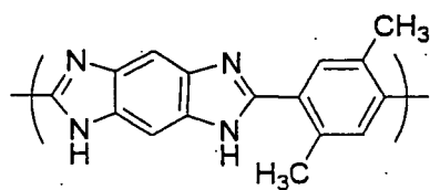
Chemical Formula 6-7
