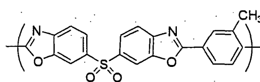
Chemical Formula 9-6
