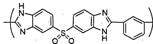
Chemical Formula 7-8
