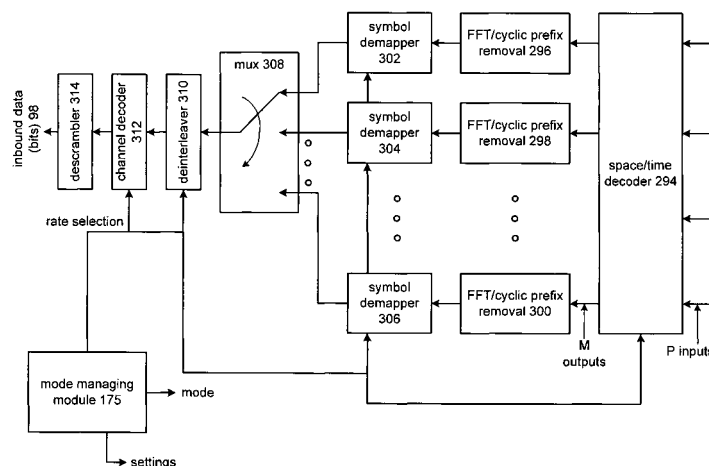
FIG. 11B WLAN receiver 250
