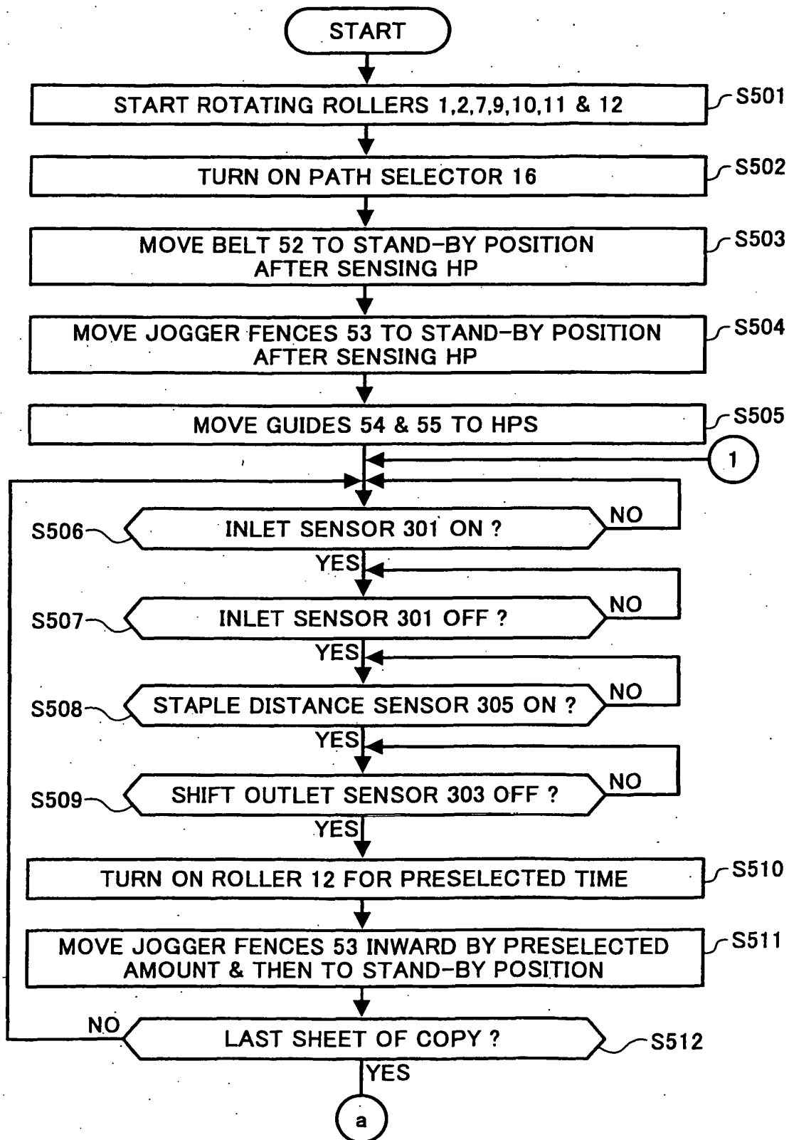
FIG. 22A CENTER STAPLE & FOLD MODE
