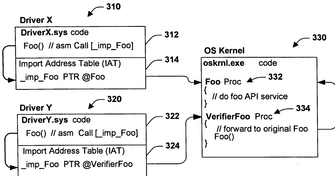
Fig. 3 Prior Art
