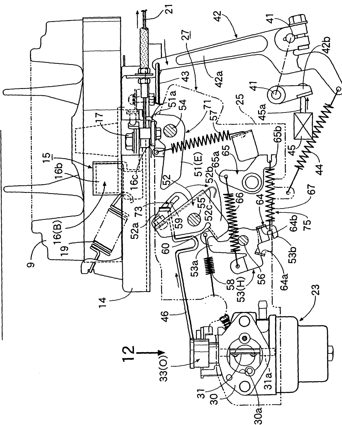
FIG.11 WHEN WARM-UP OPERATION IS FINISHED
