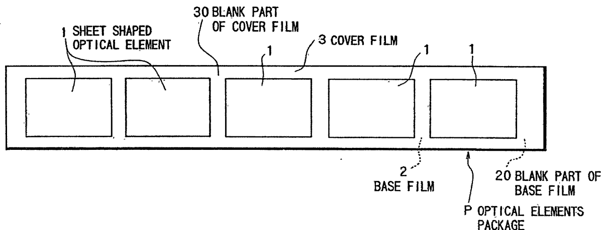
SHEET SHAPED OPTICAL ELEMENTS PACKAGE OF EXAMPLE 1 (PLANE)
