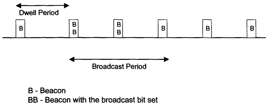
Figure 3 - Broadcast Period
