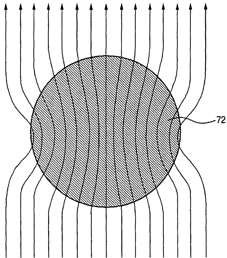
FIG. 3 IDEAL SECTIONAL SHAPE OF MAGNETIC SHIELD PLATE
