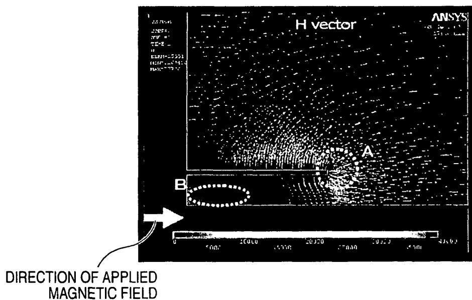
FIG. 15A CROSS SECTION
