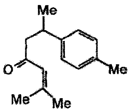
ar-Turmerone (5): Mr=216
