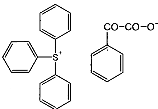
Polymerization initiator (1)
