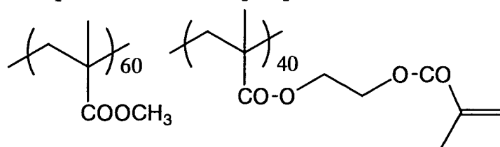
Oleophilic binder polymer (2)
