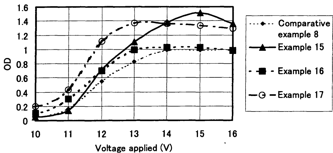
Dynamic Sensitivity characteristic curve
