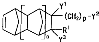
General formula (1)
