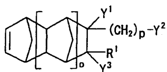
General formula (1)
