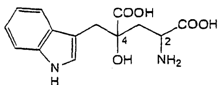
4-(indol-3-ylmethyl)-4-hydroxy-glutamic acid
