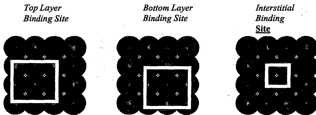
Figure 1. Molecular Modeling Study - Potential Copper Binding Sites
