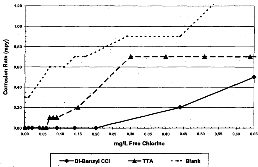
Figure 9. Corrosion Rates of Di-Benzyl CCl and TTA without Residual in the Presence of Low levels of Hypochlorite.
