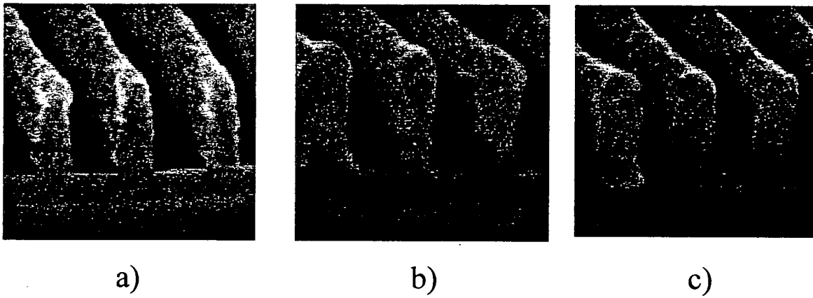
Cross-section SEM pictures after treatment with a) DI water, b) process solution 22 and c) process solution 23
