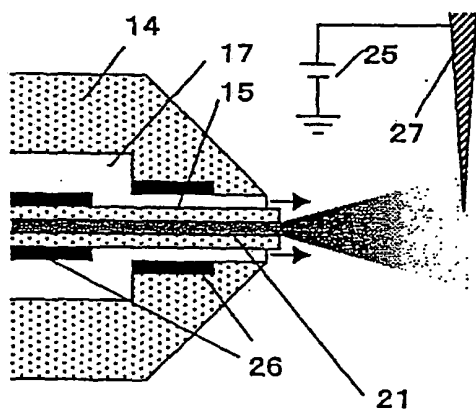
Fig. 7C PRIOR ART
