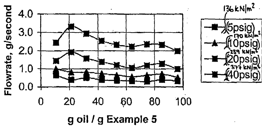
Figure 2 Packed Bed Bleaching Example
