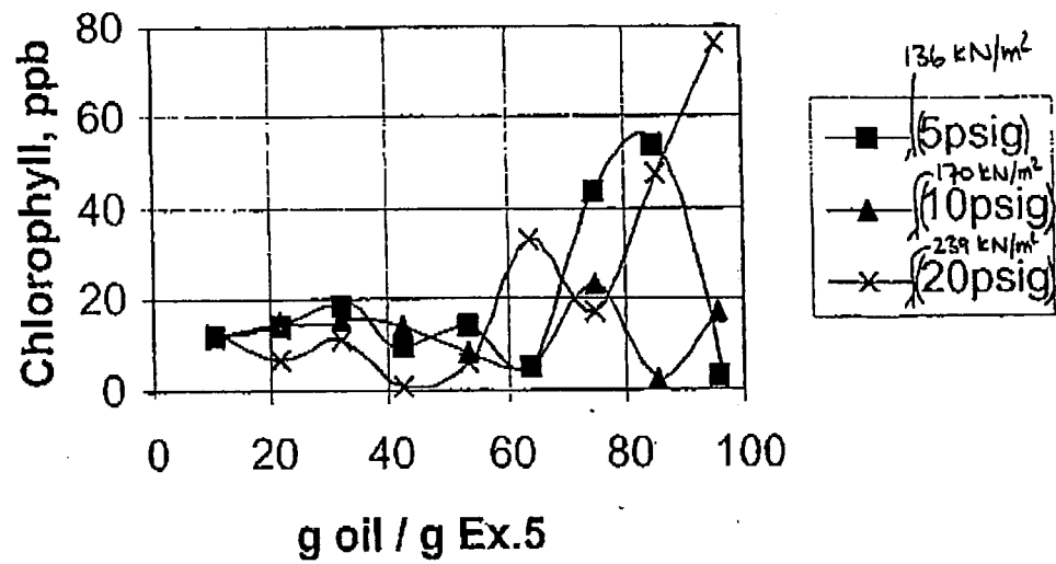
Figure 3 Packed Bed Bleaching Example
