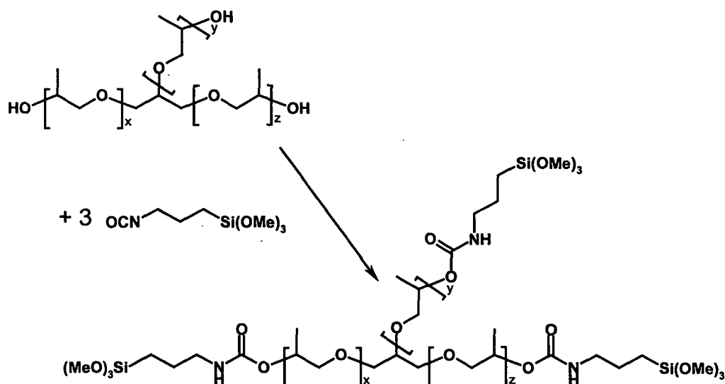
Formula 1. Synthesis of Polyether Trisilane
