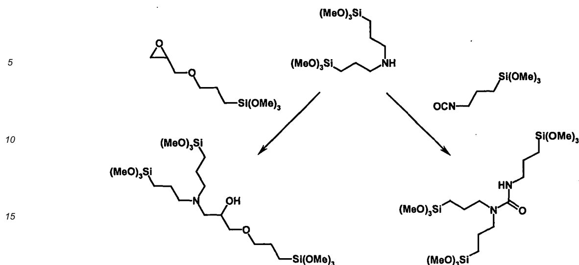
Formula 2. Synthesis of Low Molecular Weight Trisilanes
