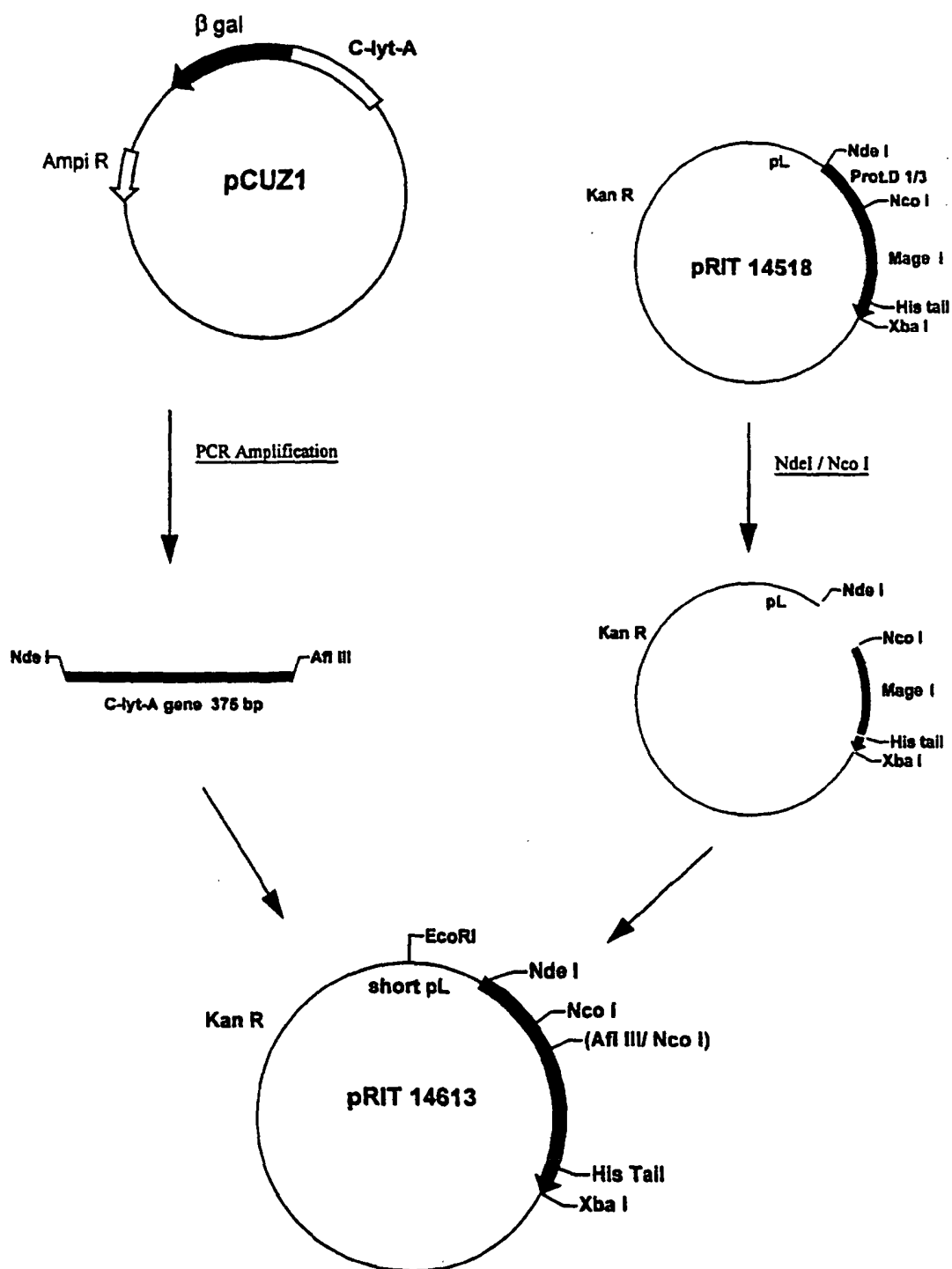
Figure 16 : construction of plasmid pRIT 14613.
