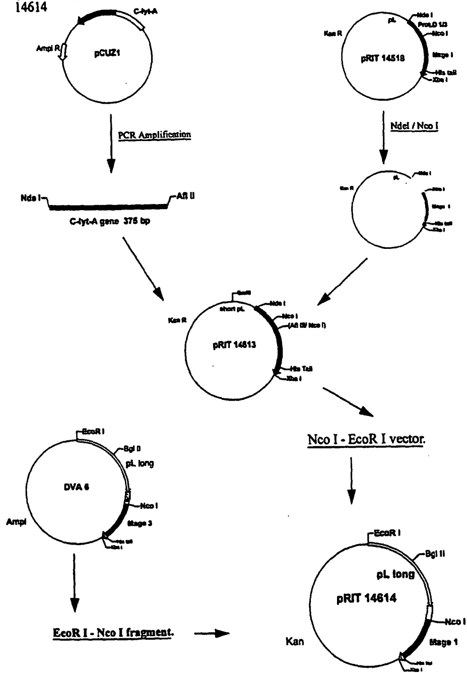
Figure 17 construction of plasmid pRIT 14614
