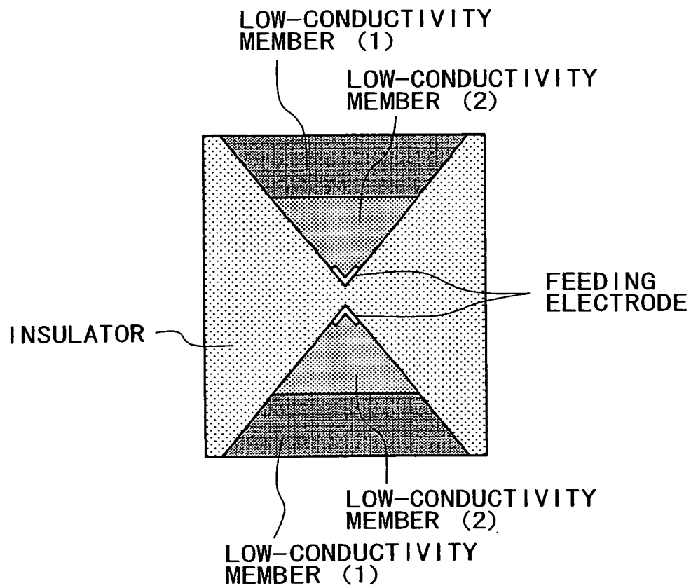
CROSS-SECTIONAL VIEW
