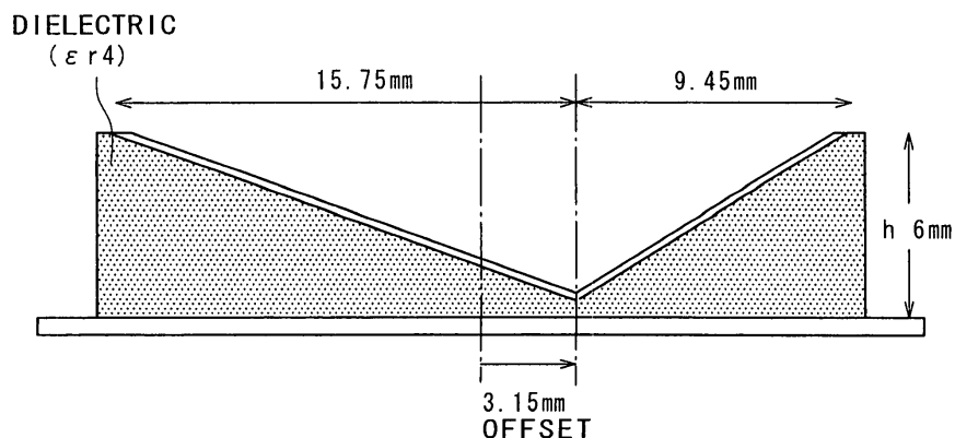
CROSS-SECTIONAL VIEW
