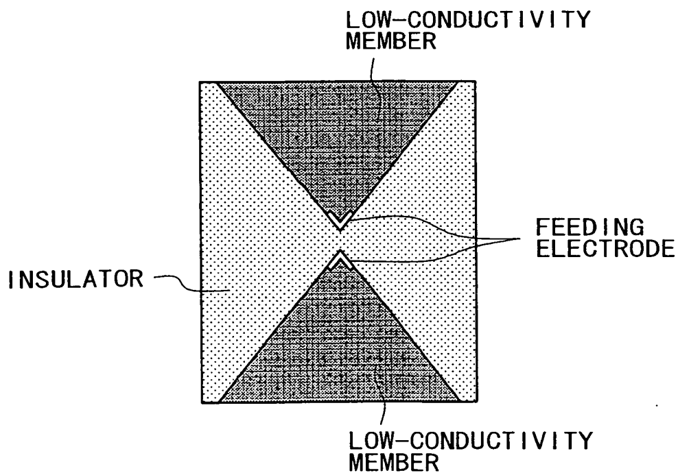
CROSS-SECTIONAL VIEW
