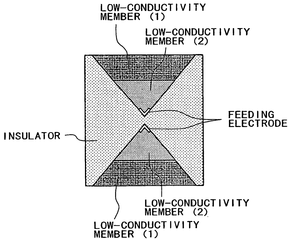
CROSS-SECTIONAL VIEW
