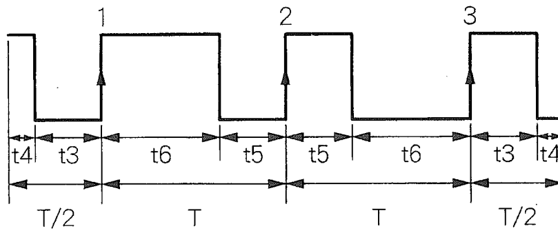
WAVEFORM C(3)
