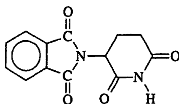
thalidomide
