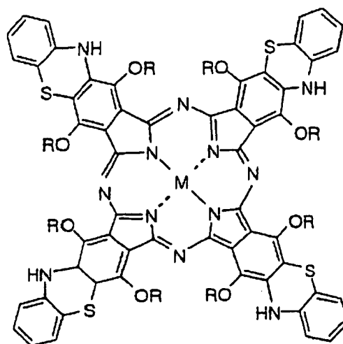
(IR-27) \text{M}=\text{VO} , \text{R}=\text{i-C}_5\text{H}_{11}
