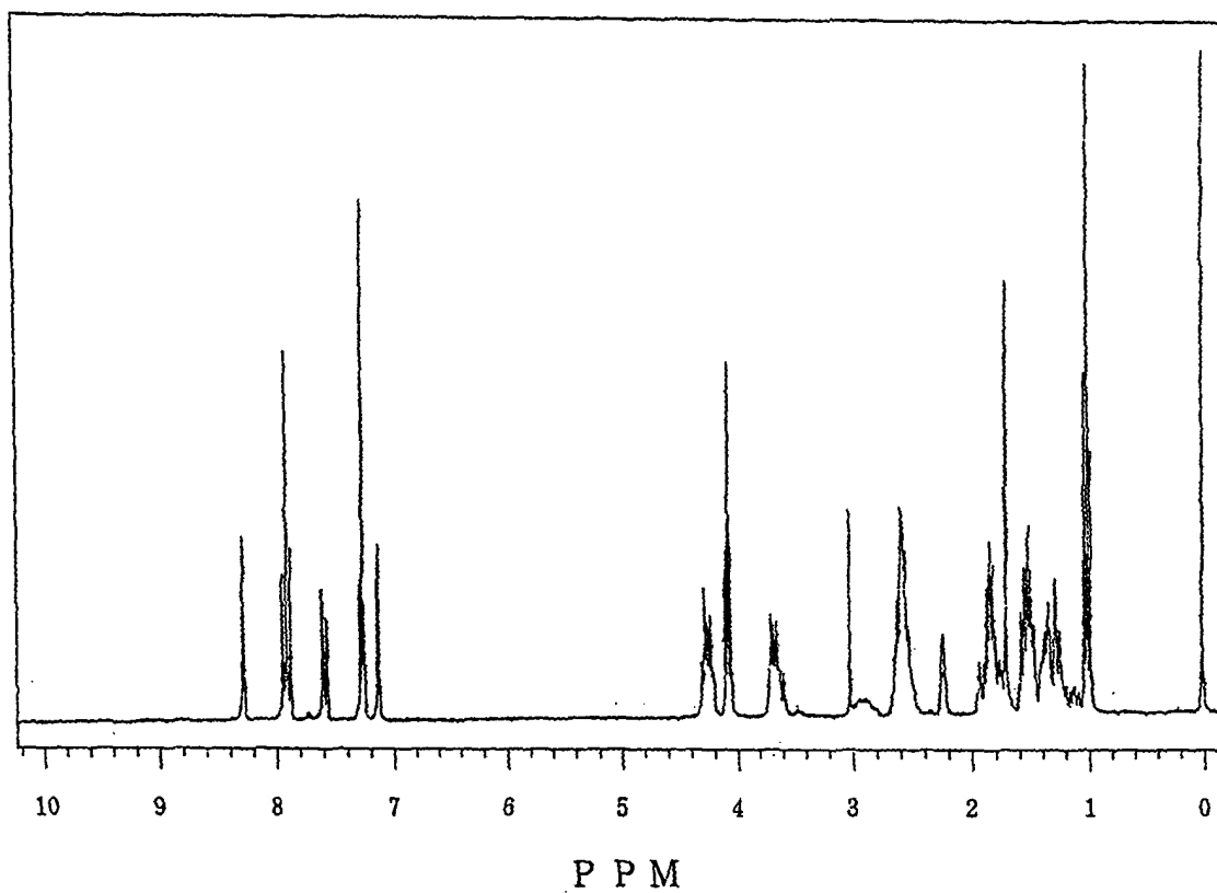
1 H-NMR spectrometry spectrum of the sulfonium salt (A-6)
