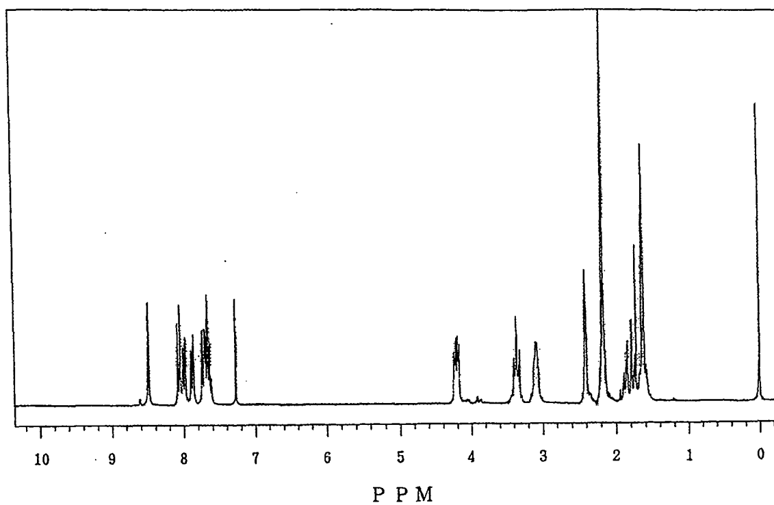
^1\text{H} -NMR spectrometry spectrum of the sulfonium salt (A-4)
