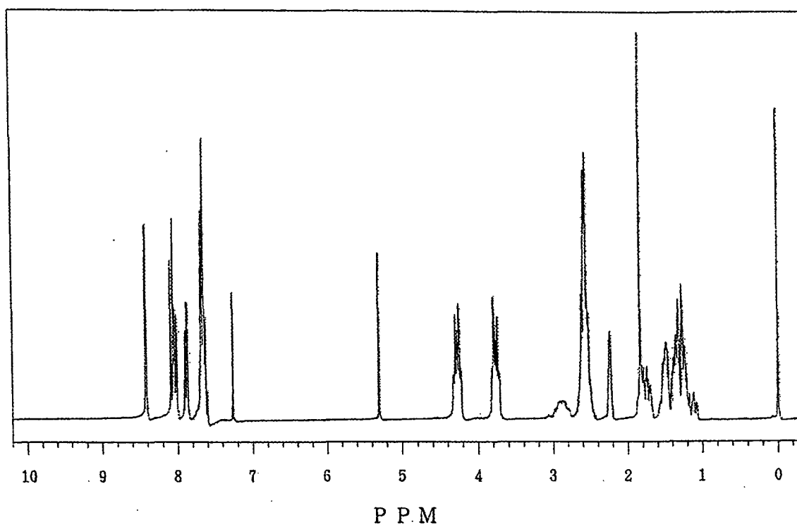
^1\text{H} -NMR spectrometry spectrum of the sulfonium salt (A-2)
