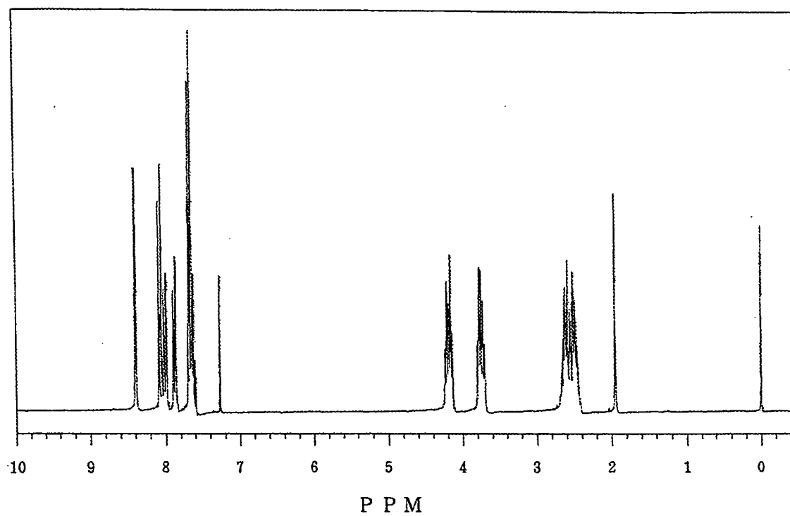
^1\text{H} -NMR spectrometry spectrum of the sulfonium salt (A-1)
