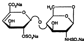
disaccharide 3
