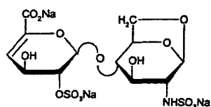
disaccharide 3
