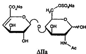
ΔIIa
