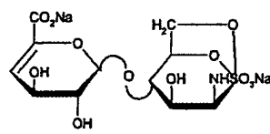
disaccharide 2
