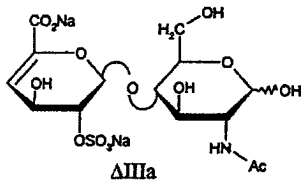
ΔIIIa
