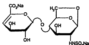
disaccharide 1
