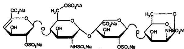
tetrasaccharide 1
