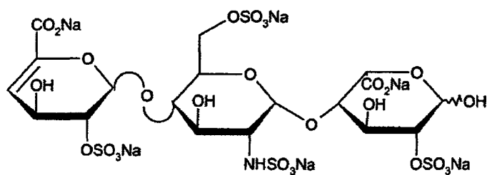
trisaccharide 1
