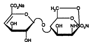
disaccharide 2
