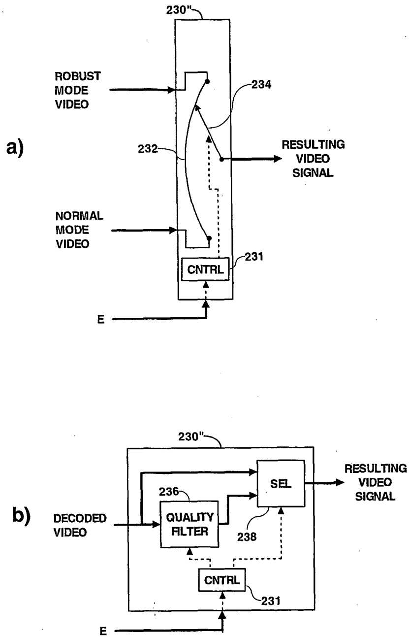
Fig. 5 Smoothing selector
