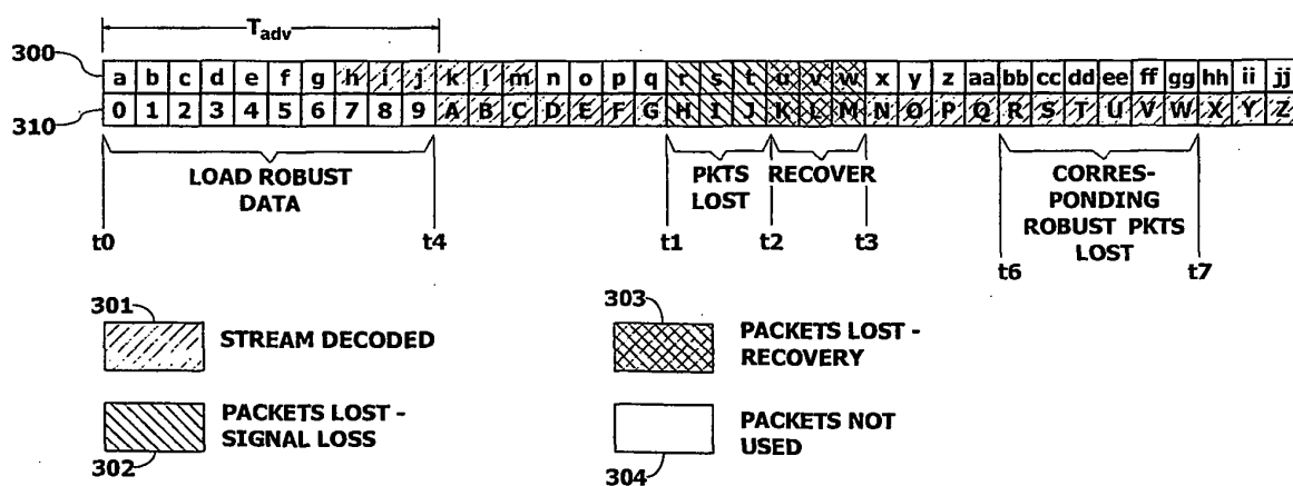
Fig. 3 Packet Streams
