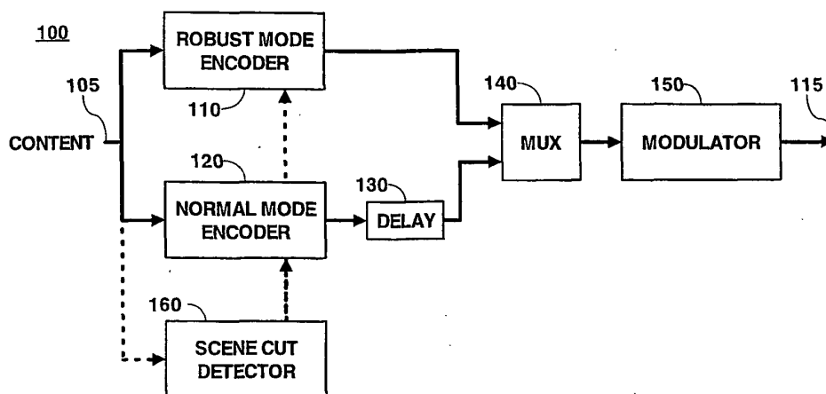
Fig. 1 Transmitter
