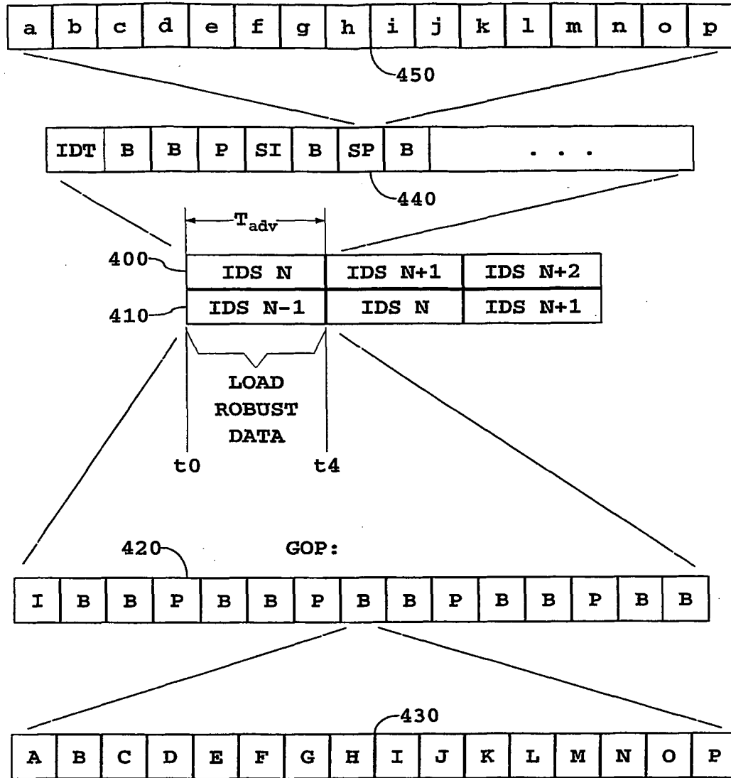
Fig. 4 GOP Streams
