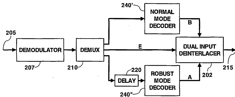
Fig. 12 Dual interlace receiver
