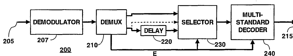
Fig. 2 Receiver
