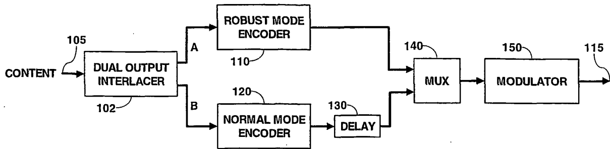
Fig. 11 Dual interlace transmitter
