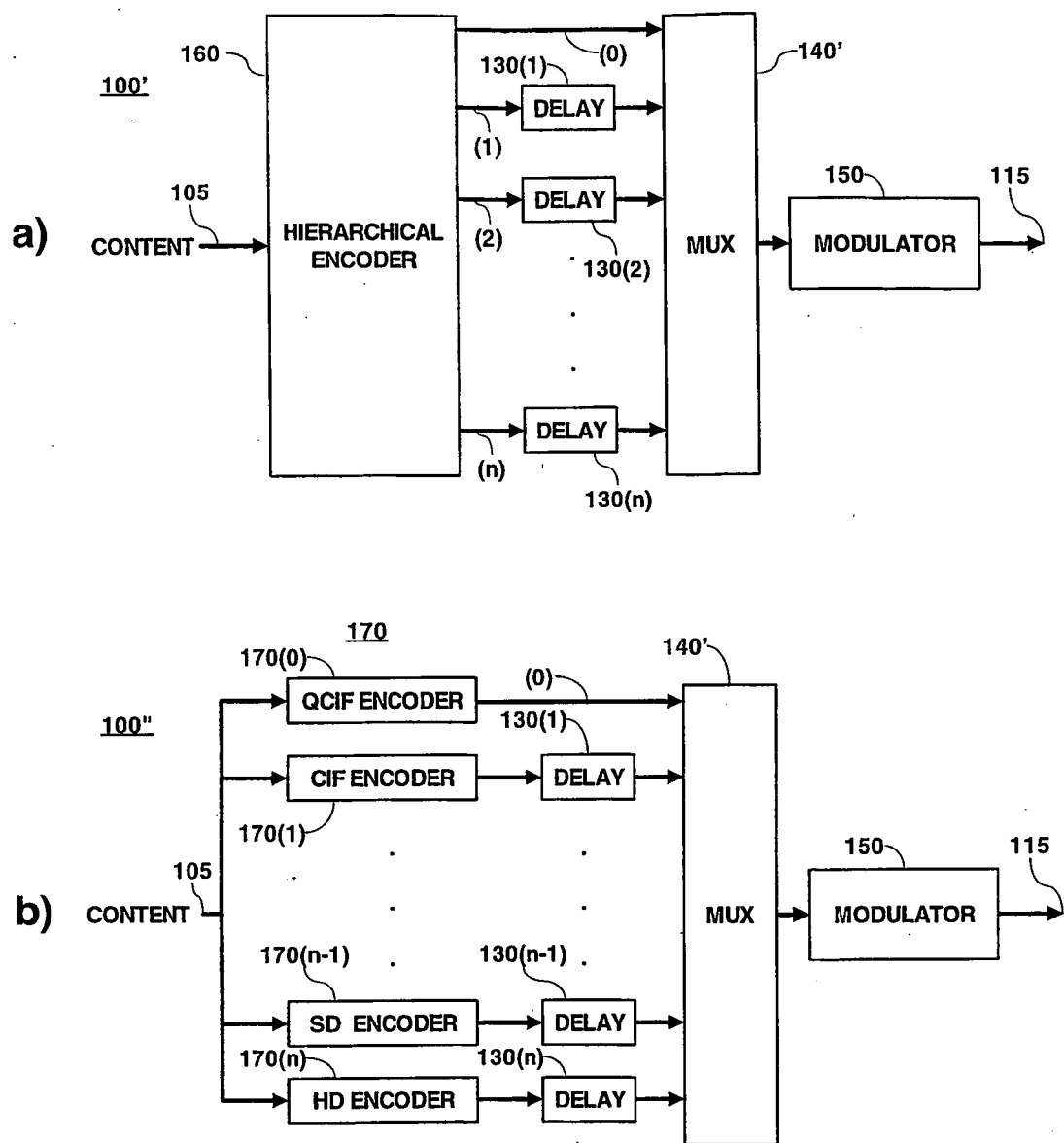
Fig. 9 Multiresolution transmitter
