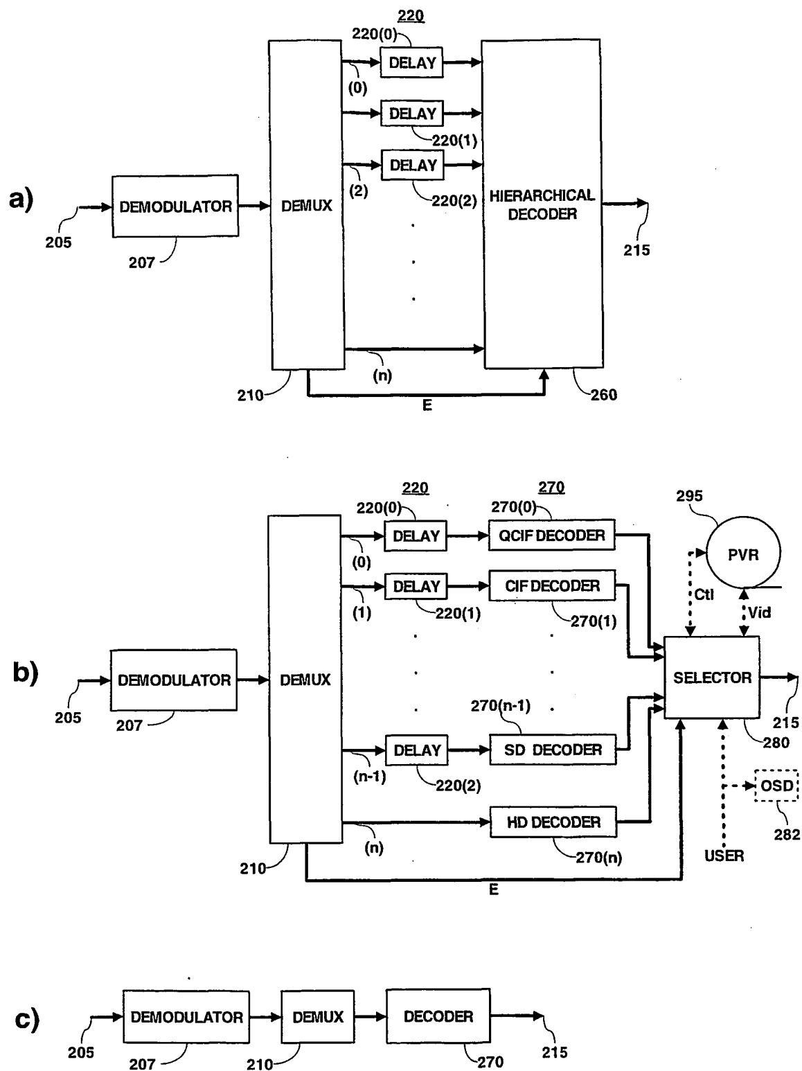
Fig. 10 Multiresolution receiver
