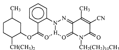
Menthyl Anthranilate Dodecyl Pyridone
