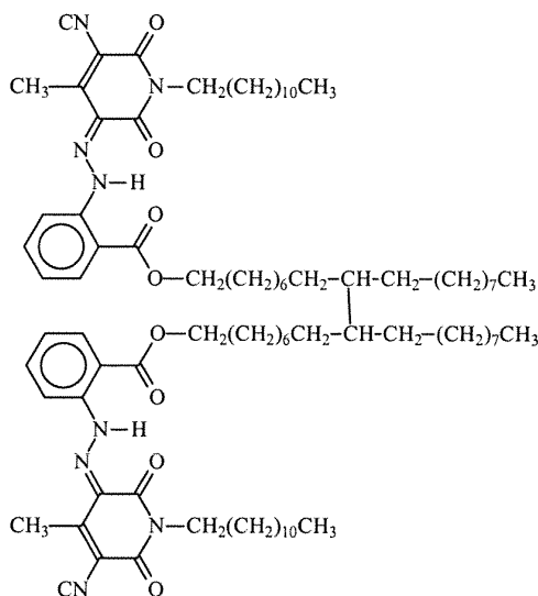
Dimer Diol Dianthranilate Bis(Dodecyl Pyridone)
