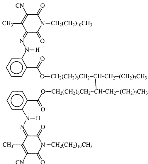
Dimer Diol Dianthranilate Bis(Dodecyl Pyridone)
