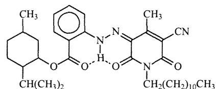
Menthyl Anthranilate Dodecyl Pyridone
