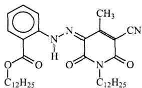
Dodecyl Anthranilate Dodecyl pyridone
