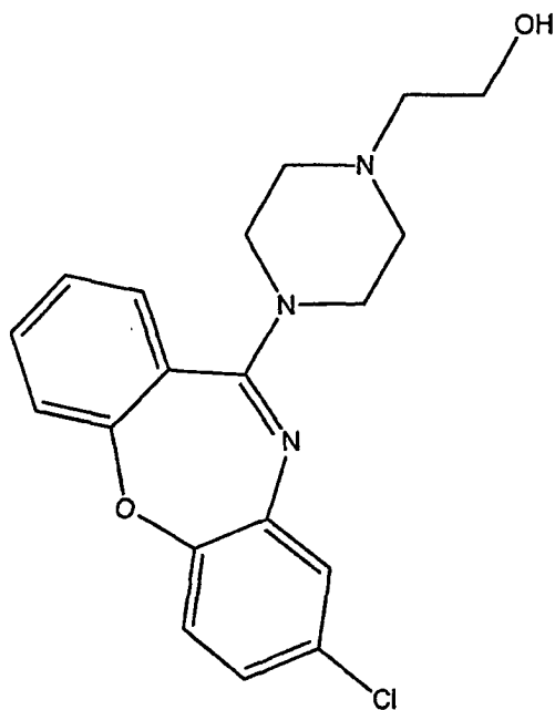
(A-7) = 8-Chloro-11-(4-(2'-hydroxyethyl)piperazin-1-yl)-dibenzo[b,f][1,4]oxazepine.
