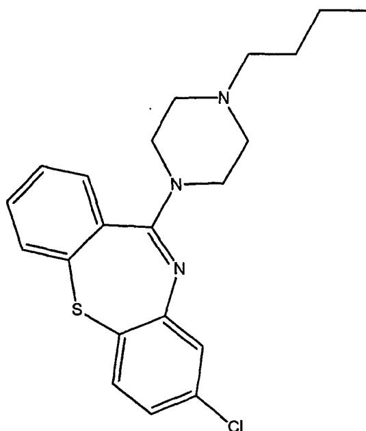
(A-16) = 8-Chloro-11-(4-butylpiperazin-1-yl)-dibenzo[b,f][1,4]thiazepine.
