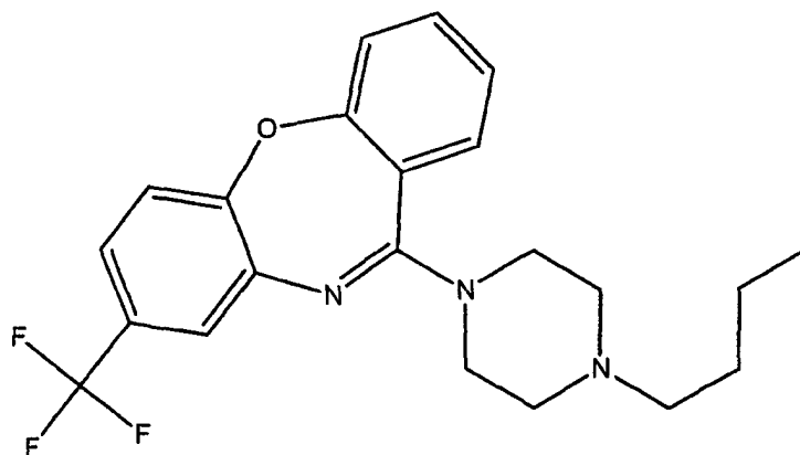
(A-5) = 8-Trifluoromethyl-11-(4-butylpiperazin-1-yl)-dibenzo[b,f][1,4]oxazepine;
