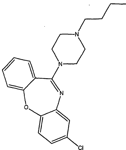
(A-10) = 8-Chloro-11-(4-butylpiperazin-1-yl)-dibenzo[b,f][1,4]oxazepine;
