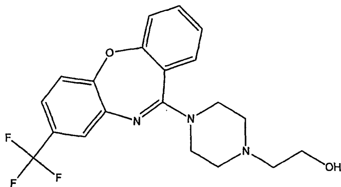
(A-2) = 8-Trifluoromethyl-11-(4-(2'-hydroxyethyl)piperazin-1-yl)-dibenzo[b,f][1,4]oxazepine;
