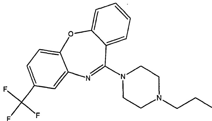
(A-3) = 8-Trifluoromethyl-11-(4-propylpiperazin-1-yl)-dibenzo[b,f][1,4]oxazepine;
