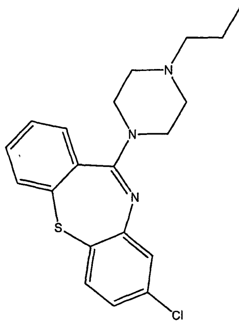
(A-14) = 8-Chloro-11-(4-propylpiperazin-1-yl)-dibenzo[b,f][1,4]thiazepine;
