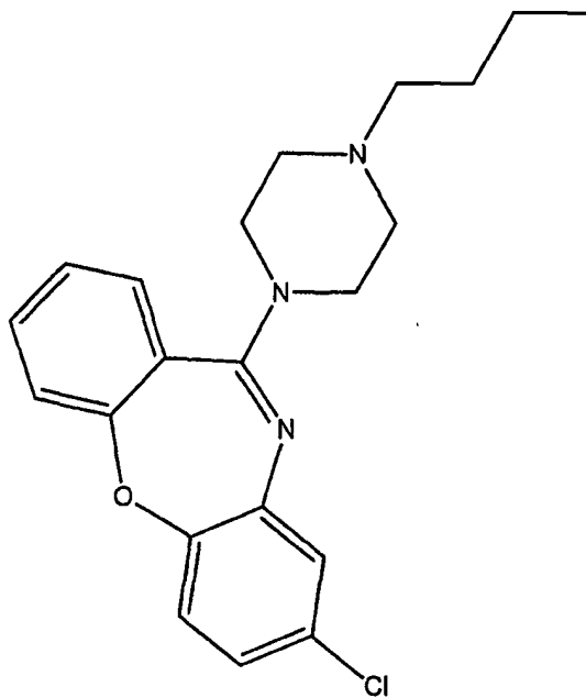
(A-10) = 8-Chloro-11-(4-butylpiperazin-1-yl)-dibenzo[b,f][1,4]oxazepine;
