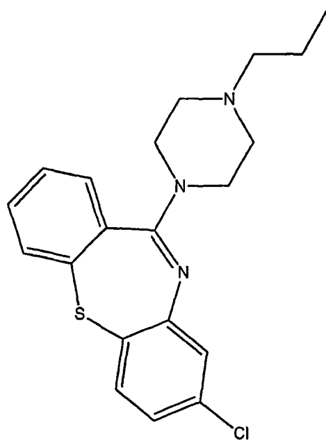
(A-14) = 8-Chloro-11-(4-propylpiperazin-1-yl)-dibenzo[b,f][1,4]thiazepine;
