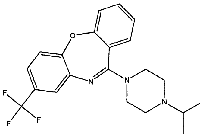
(A-4) = 8-Trifluoromethyl-11-(4-isopropylpiperazin-1-yl)-dibenzo[b,f][1,4]oxazepine;
