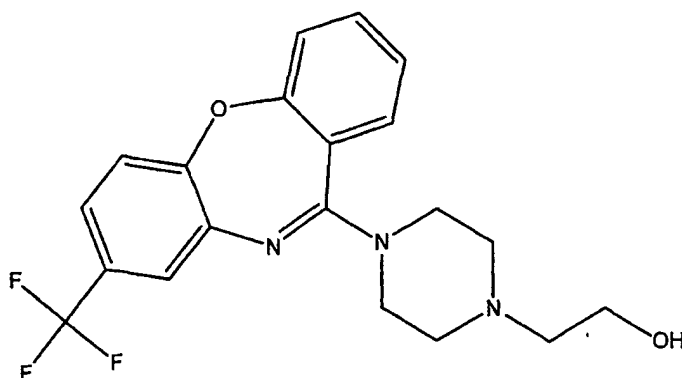
(A-2) = 8-Trifluoromethyl-11-(4-(2'-hydroxyethyl)piperazin-1-yl)-dibenzo[b,f][1,4]oxazepine;
