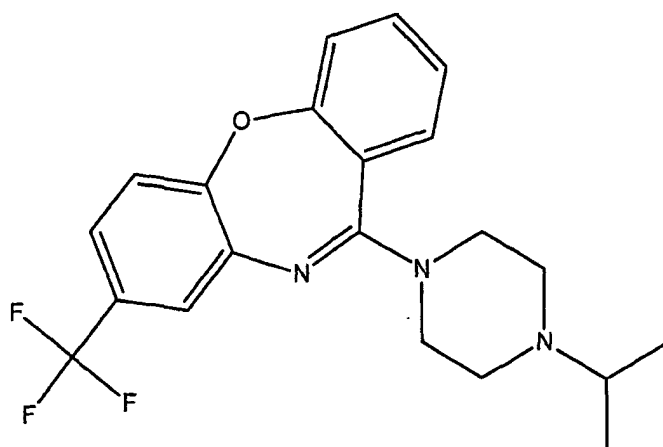
(A-4) = 8-Trifluoromethyl-11-(4-isopropylpiperazin-1-yl)-dibenzo[b,f][1,4]oxazepine;
