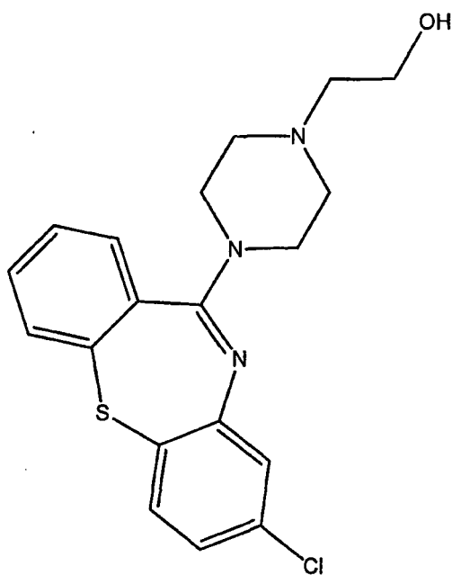
(A-13) = 8-Chloro-11-(4-(2'-hydroxyethyl)piperazin-1-yl)-dibenzo[b,f][1,4]thiazepine;
