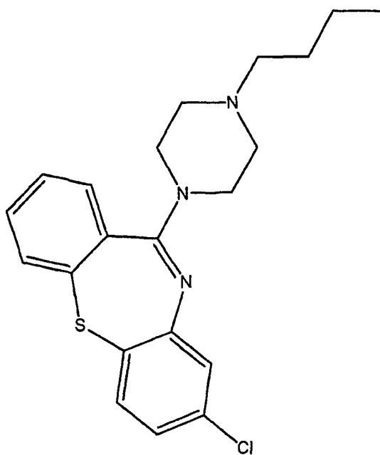
(A-16) = 8-Chloro-11-(4-butylpiperazin-1-yl)-dibenzo[b,f][1,4]thiazepine.
