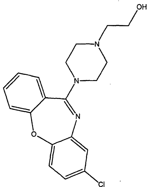
(A-7) = 8-Chloro-11-(4-(2'-hydroxyethyl)piperazin-1-yl)-dibenzo[b,f][1,4]oxazepine;
