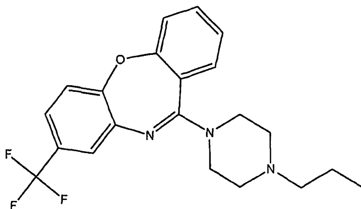
(A-3) = 8-Trifluoromethyl-11-(4-propylpiperazin-1-yl)-dibenzo[b,f][1,4]oxazepine;
