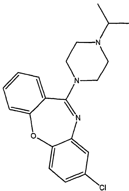
(A-9) = 8-Chloro-11-(4-isopropylpiperazin-1-yl)-dibenzo[b,f][1,4]oxazepine;
