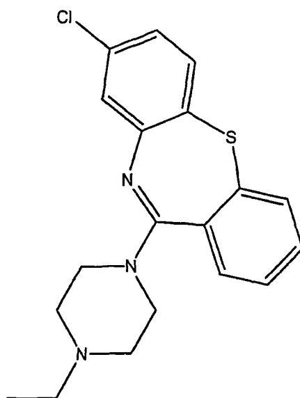
(A-12) = 8-Chloro-11-(4-ethylpiperazin-1-yl)-dibenzo [b,f][1,4]thiazepine;
