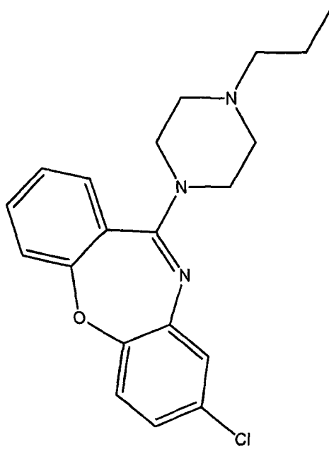
(A-8) = 8-Chloro-11-(4-propylpiperazin-1-yl)-dibenzo[b,f][1,4]oxazepine;
