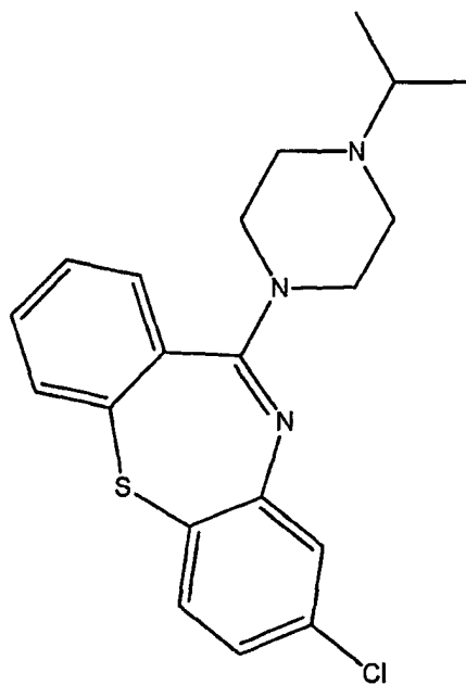
(A-15) = 8-Chloro-11-(4-isopropylpiperazin-1-yl)-dibenzo[b,f][1,4]thiazepine; and
