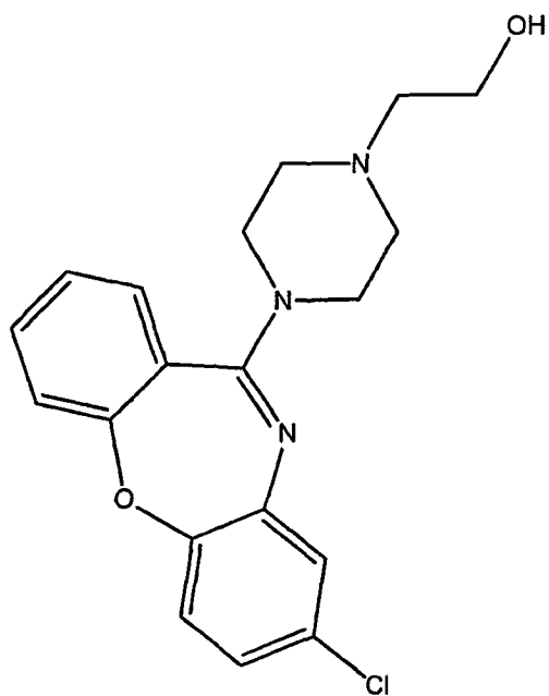
(A-7) = 8-Chloro-11-(4-(2'-hydroxyethyl)piperazin-1-yl)-dibenzo[b,f][1,4]oxazepine;
