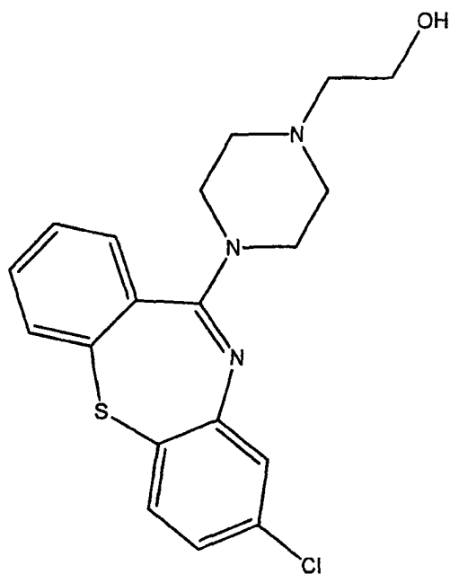
(A-13) = 8-Chloro-11-(4-(2'-hydroxyethyl)piperazin-1-yl)-dibenzo[b,f][1,4]thiazepine;
