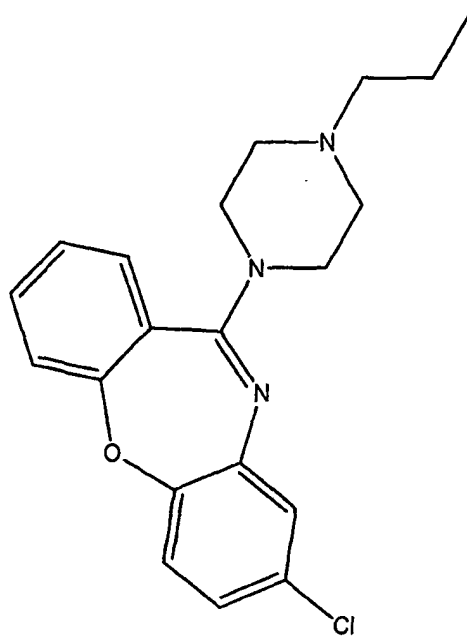
(A-8) = 8-Chloro-11-(4-propylpiperazin-1-yl)-dibenzo[b,f][1,4]oxazepine;
