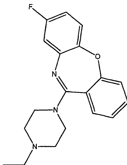
(A-11) = 8-Fluoro-11-(4-ethylpiperazin-1-yl)-dibenzo[b,f][1,4]oxazepine;
