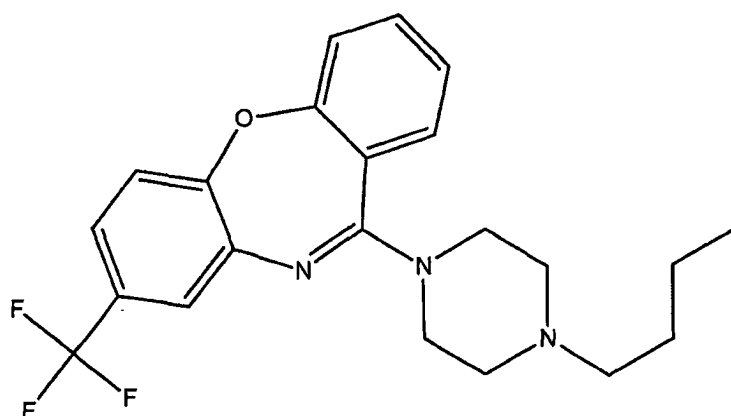
(A-5) = 8-Trifluoromethyl-11-(4-butylpiperazin-1-yl)-dibenzo[b,f][1,4]oxazepine;
