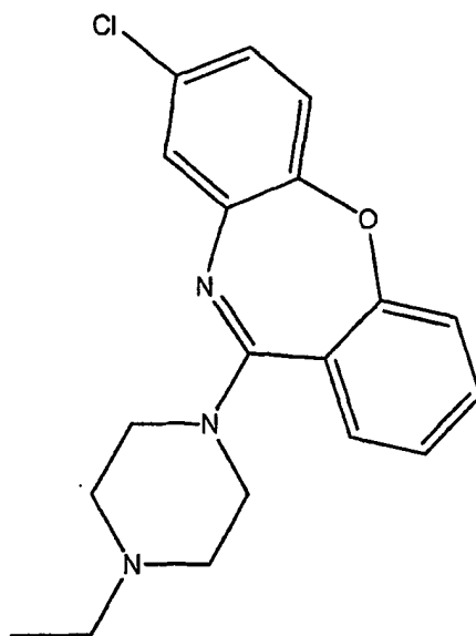
(A-6) = 8-Chloro-11-(4-ethylpiperazin-1-yl)-dibenzo[b,f][1,4]oxazepine;
