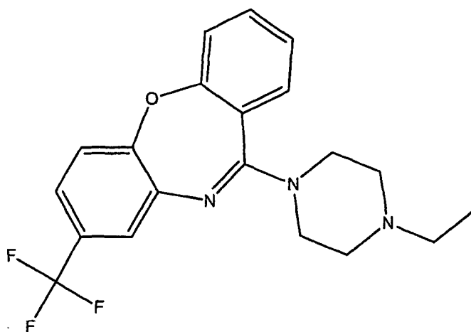
(A-1) = 8-Trifluoromethyl-11-(4-ethylpiperazin-1-yl)-dibenzo[b,f][1,4]oxazepine;
