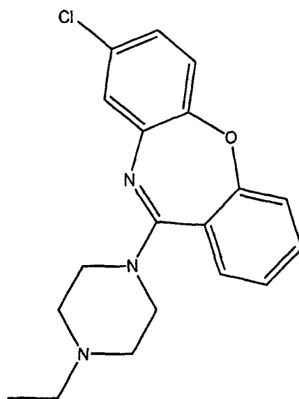
(A-6) = 8-Chloro-11-(4-ethylpiperazin-1-yl)-dibenzo[b,f][1,4]oxazepine;
