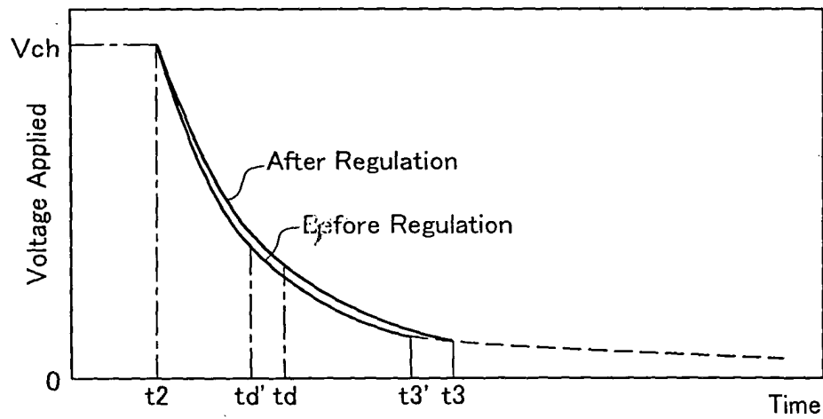
Applied Voltage of Piezoelectric Element in Time Domain (Discharge Time)
