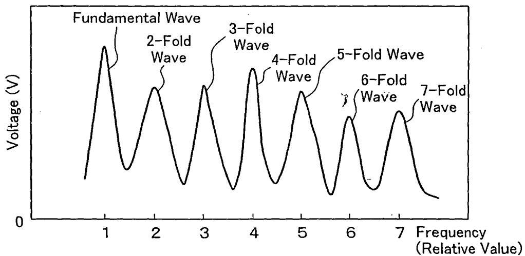
Applied Voltage of Piezoelectric Element in Frequency Domain
