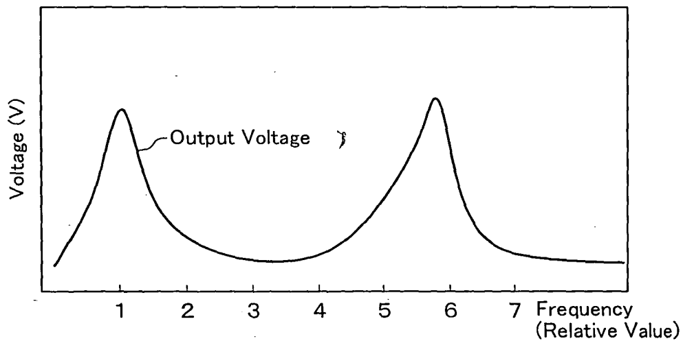
Output Voltage of Sensor In Frequency Domain
