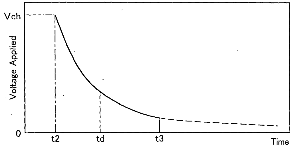
Applied Voltage of Piezoelectric Element in Time Domain (Discharge Time)
