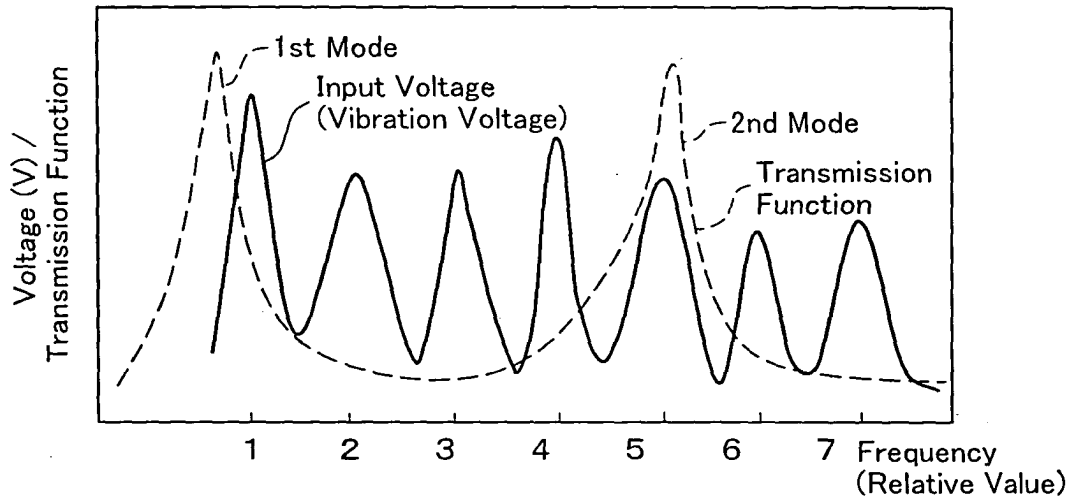
Vibration Voltage and Transmission Function Of Sensor In Frequency Domain
