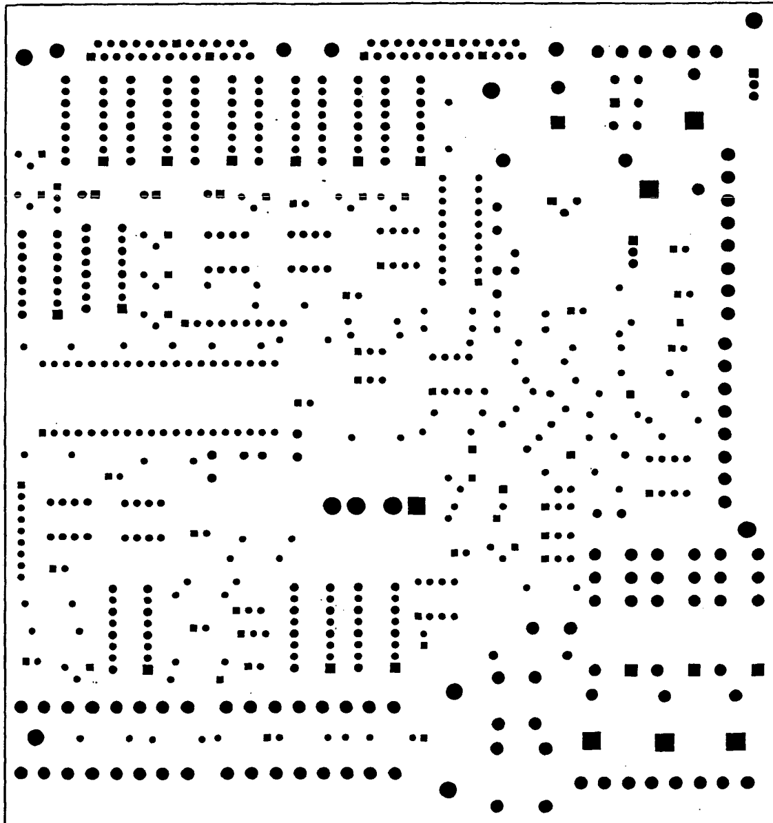
P.C.B. Solder Mask
