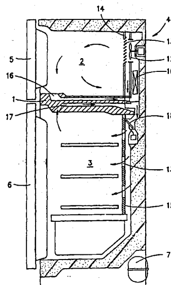
FIG.1 (PRIOR ART)
