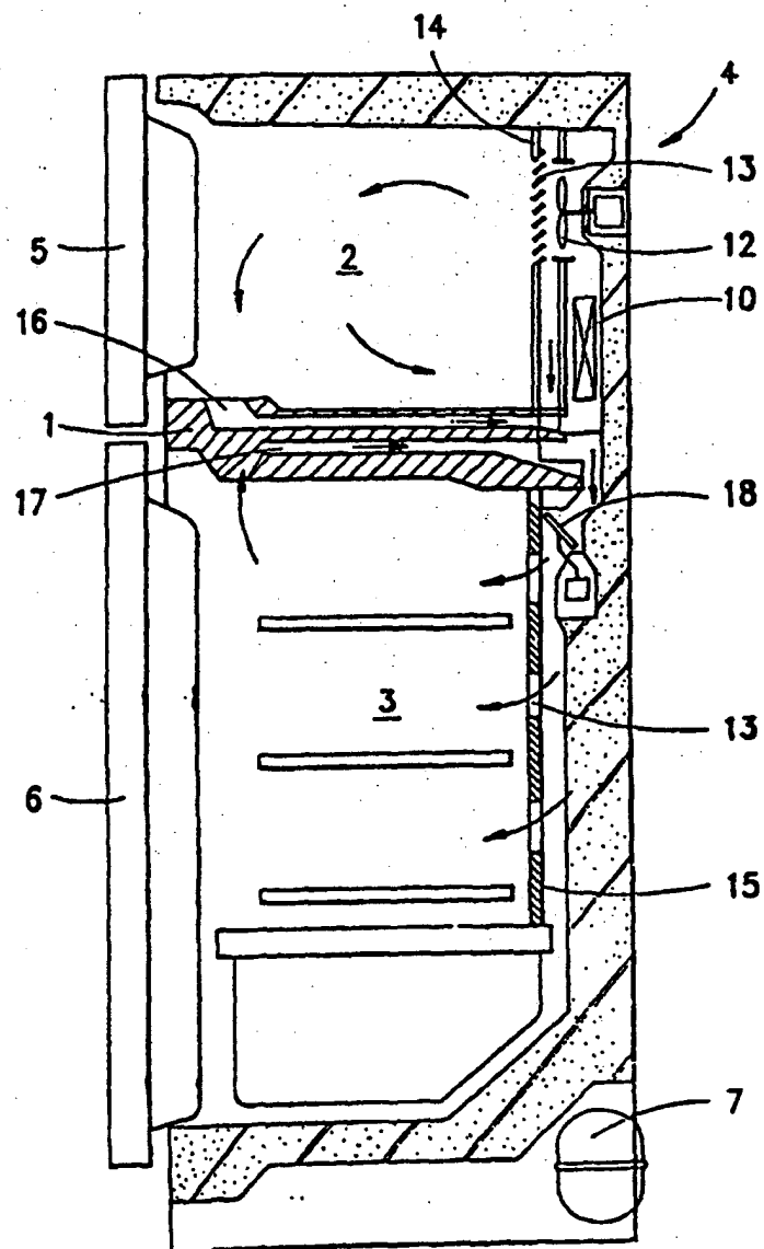
FIG. 1 (PRIOR ART)
