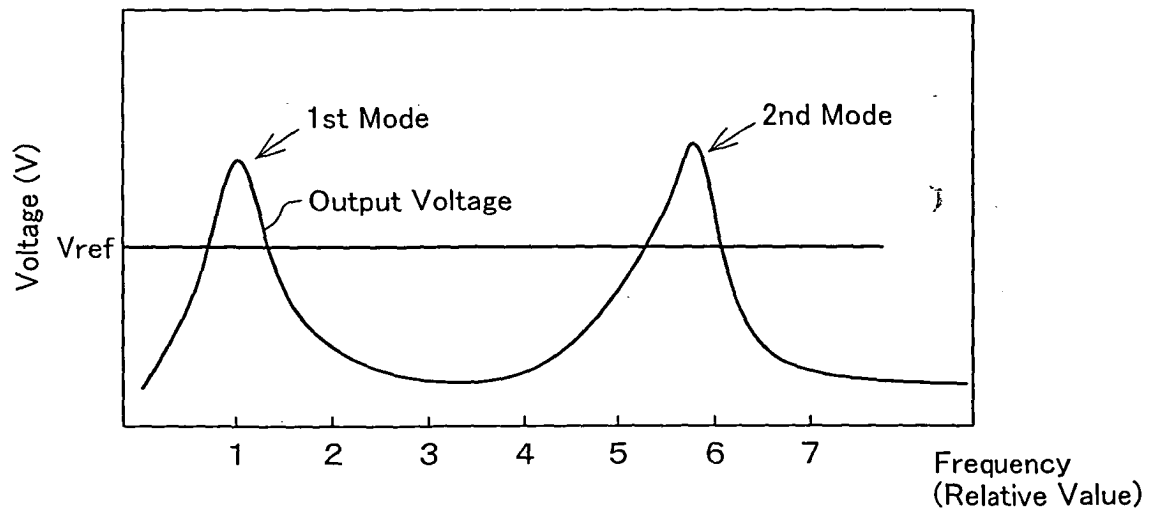
Output Voltage of Sensor in Frequency Domain
