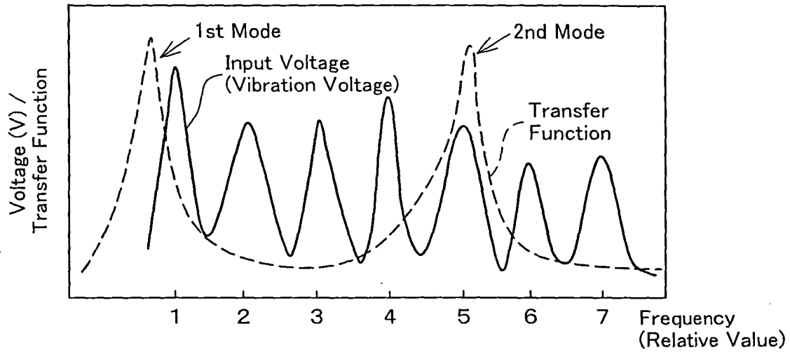
Vibration Voltage And Transfer Function of Sensor in Frequency Domain (Before Regulation)
