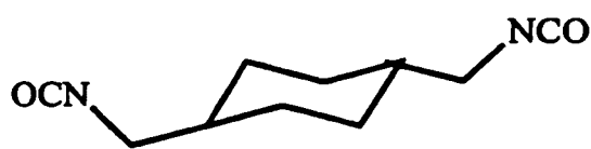
trans-1,4-bis(isocyanatomethyl)- cyclohexane Formula III
