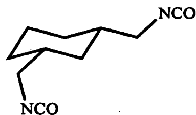
cis-1,3-bis(isocyanatomethyl)- cyclohexane Formula II
