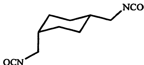
cis-1,4-bis(isocyanatomethyl)- cyclohexane Formula IV
