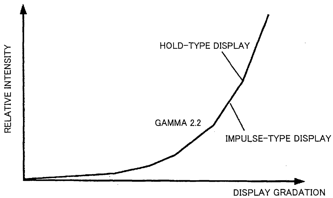
GAMMA CHARACTERISTICS OF LIQUID CRYSTAL DISPLAY
