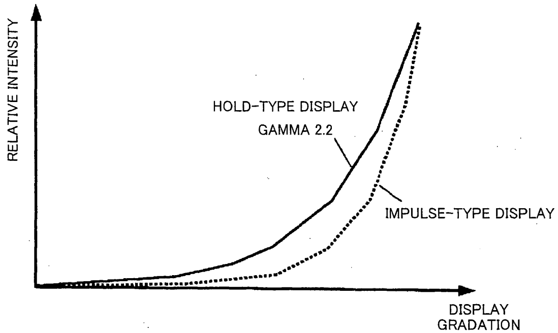
GAMMA CHARACTERISTICS OF LIQUID CRYSTAL DISPLAY
