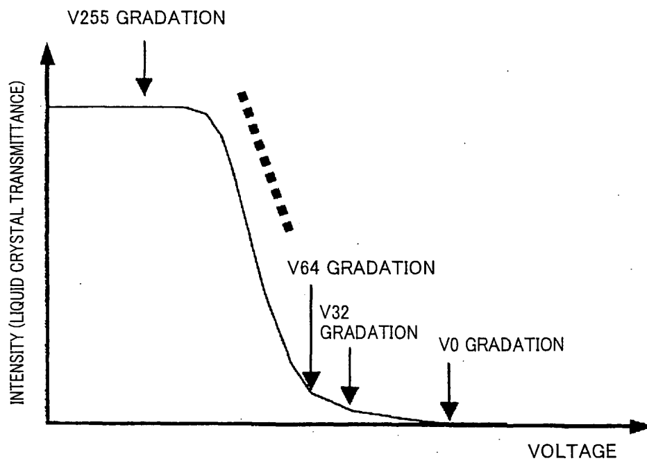
V-T CHARACTERISTICS OF LIQUID CRYSTAL DISPLAY PANEL AND VOLTAGES
