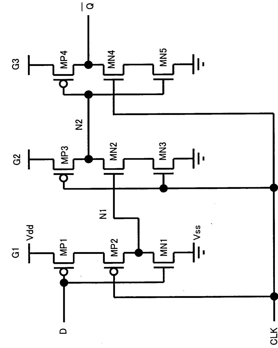
Dynamic Type Flip-Flop Circuit
