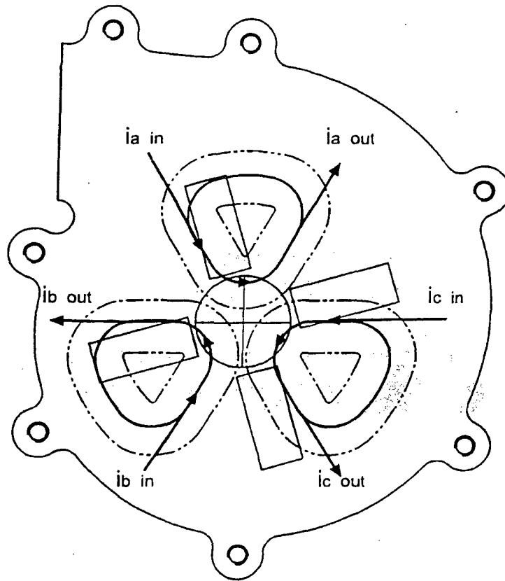
Cover coil superimposed by rectangular magnets.
