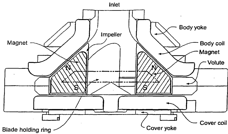
Sketch of the pump cross-section.
