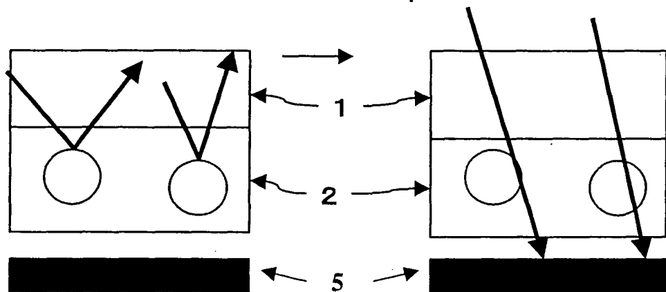
(b) Mirror Diffuse Reflection \leftrightarrow Absorption
