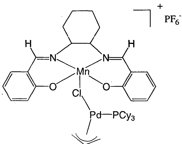
cationic metal-pair complex 4
