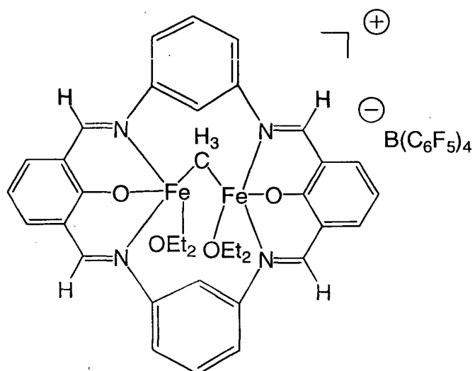
cationic metal-pair complex 1
