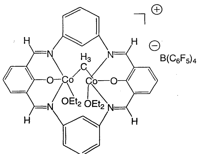
cationic metal-pair complex 2
