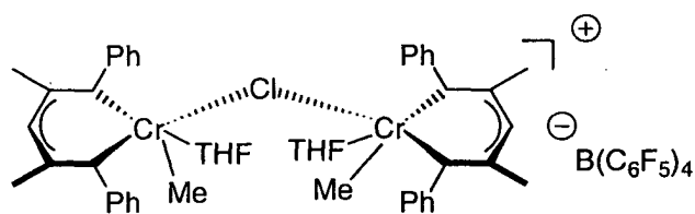
cationic metal-pair complex 5
