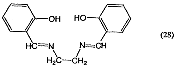
[Chemical Formula 6]
