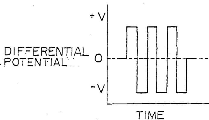
FIG. 1C DRIVE WAVEFORM OF RECTANGULAR WAVE
