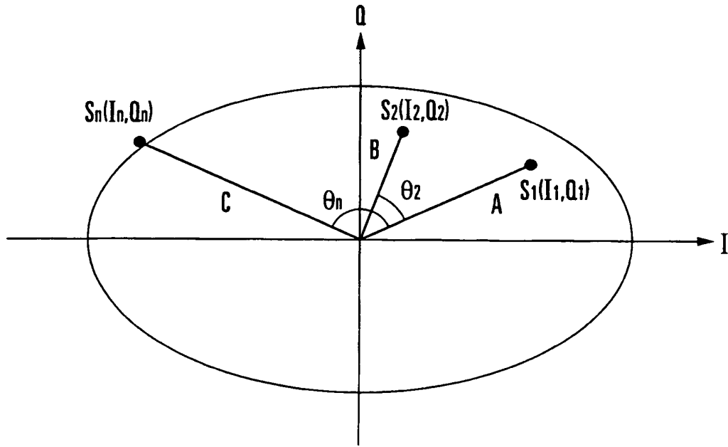
FIG. 9 PRIOR ART
