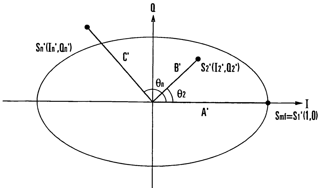
FIG. 10 PRIOR ART
