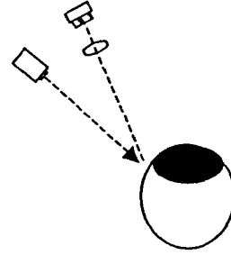
DETECTED QUANTITY OF LIGHT W_1 > W_1 WHEN PUPIL MOVES AWAY FROM OPTICAL-AXIS DIRECTION
