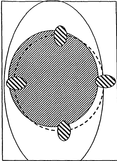
WHEN PUPIL MOVES, DETECTED QUANTITY OF LIGHT IS CHANGED AT RING-PORTION-DETECTION LIGHT-RECEIVING SECTIONS
