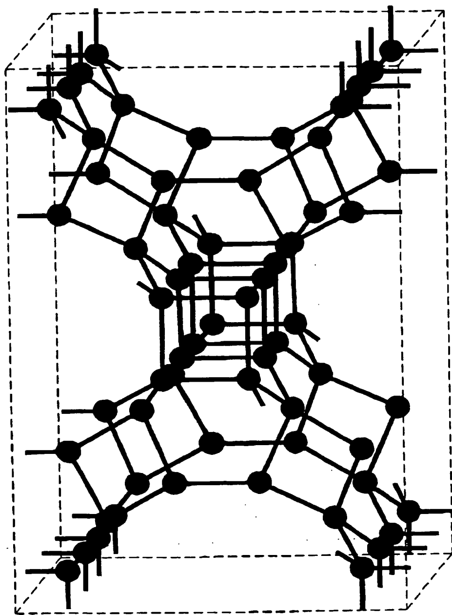
Unit cell of zeolite ITQ-24
