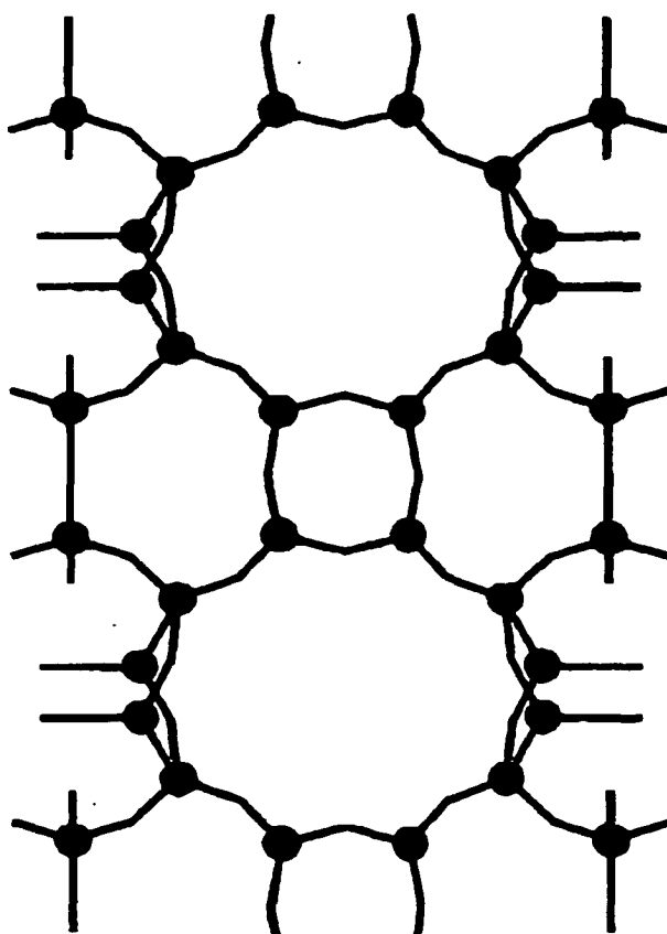
View of the channels formed by 10 tetrahedrons of zeolite ITQ-24
