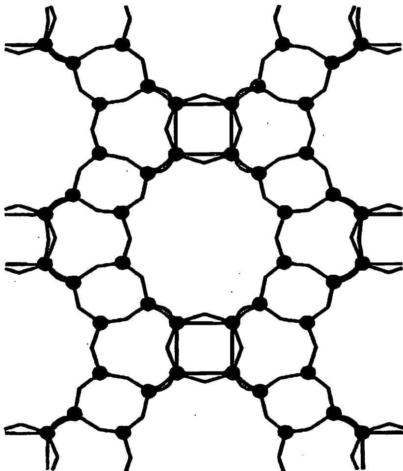
View of the rectilinear channels formed by 12 tetrahedrons of zeolite ITQ-24
