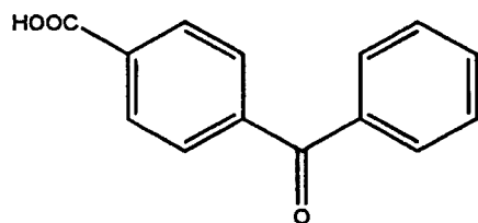
Compound 15
