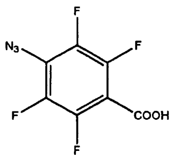
Compound 21
