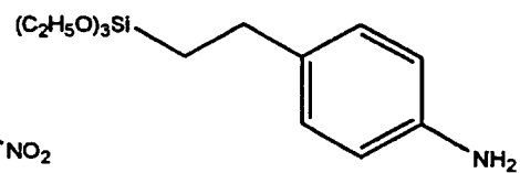
Compound 18
