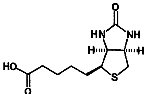
Biotin
