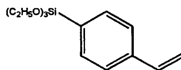
Compound 16
