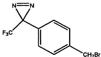
Compound 5
