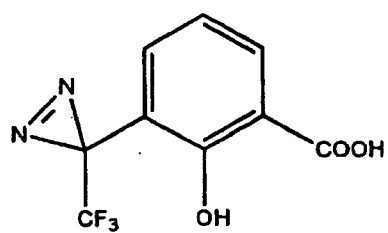
Compound 23
