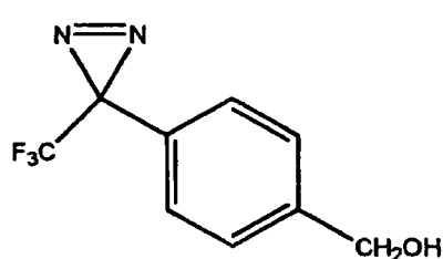
Compound 4
