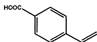
Compound 13
