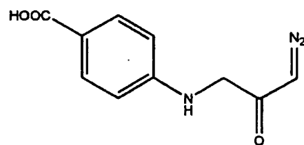
Compound 12
