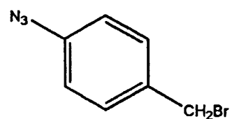
Compound 10
