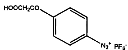
Compound 11
