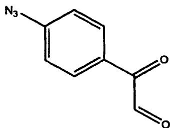
Compound 25
