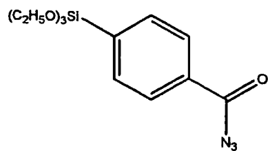
Compound 19
