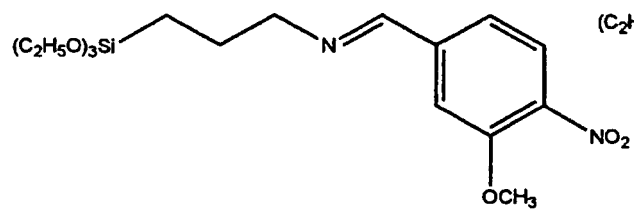
Compound 18
