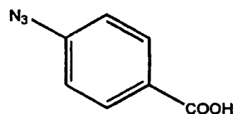
Compound 6
