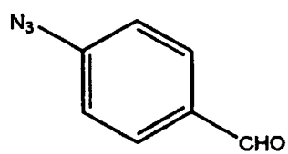
Compound 7
