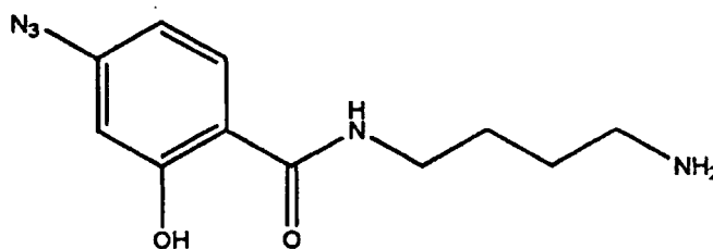
Compound 26
