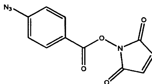
Compound 8
