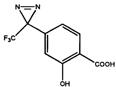
Compound 22
