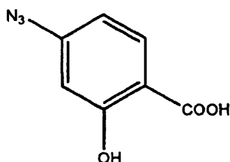
Compound 27
