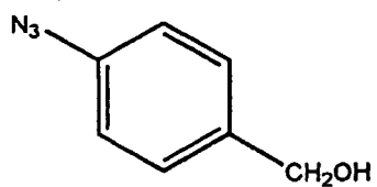
Compound 9
