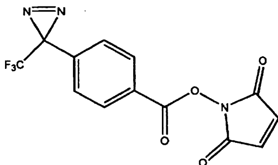
Compound 3
