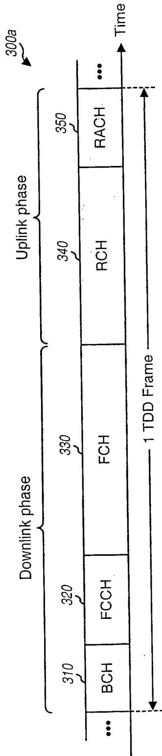
TDD-TDM Frame Structure
